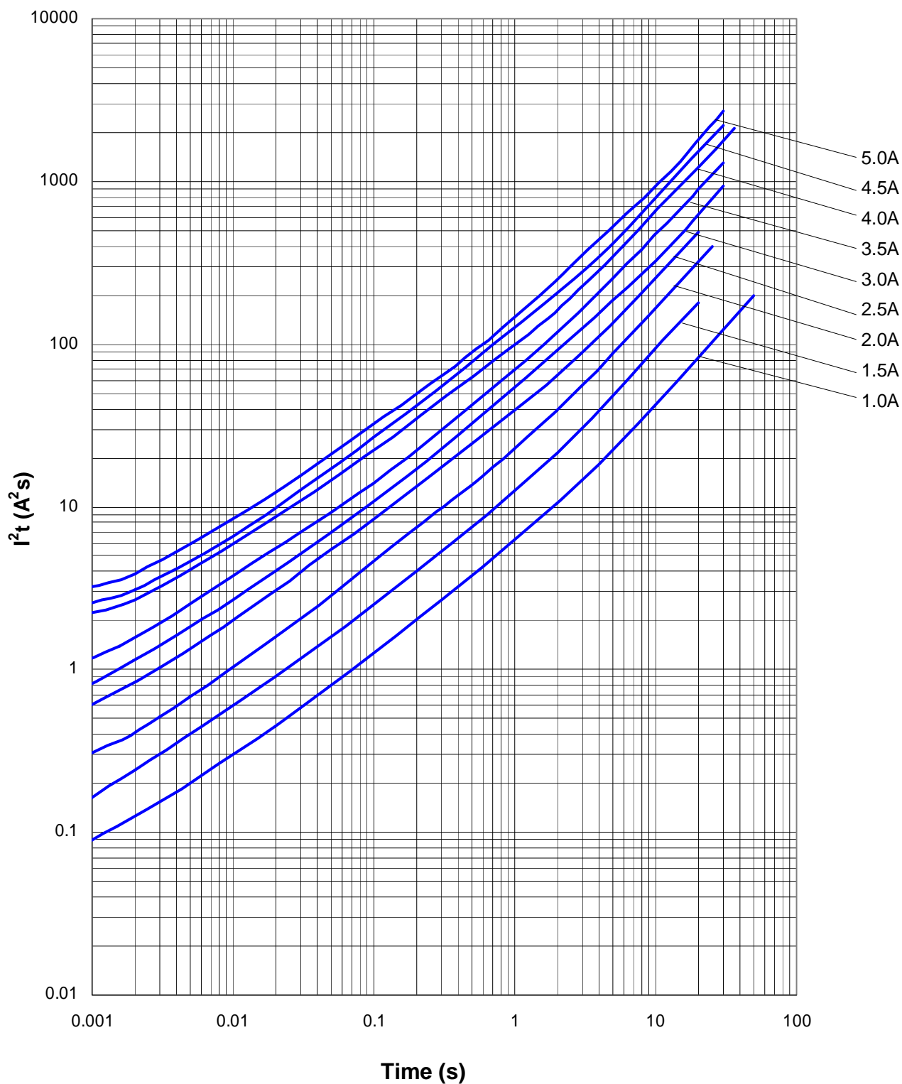
Average I^2t vs. t Curves
