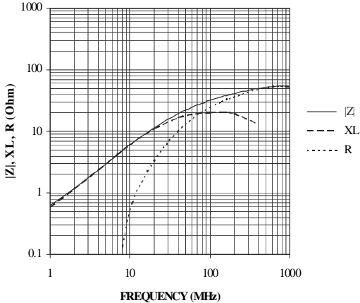
MCP1206F300
